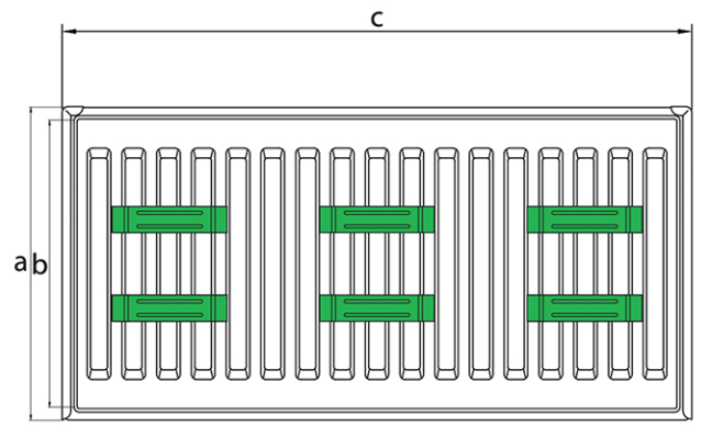
6 hangers; 1700/...../3000 mm
