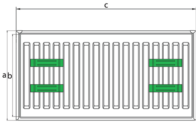
4 hangers; 400/...../1600 mm
